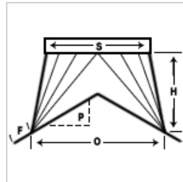
Ridge Roof
