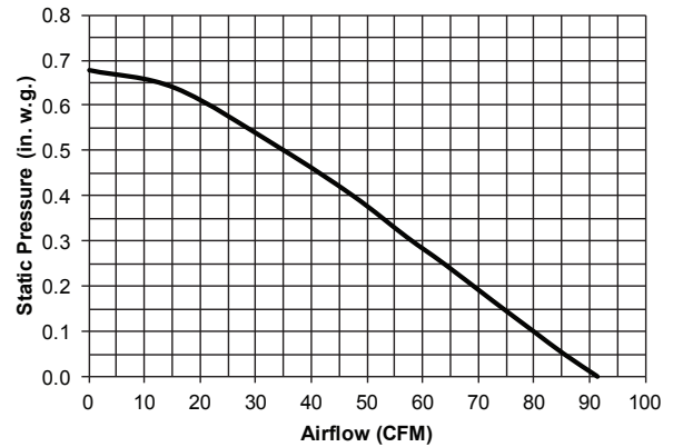
MODEL EZ80N - 4" DUCT
