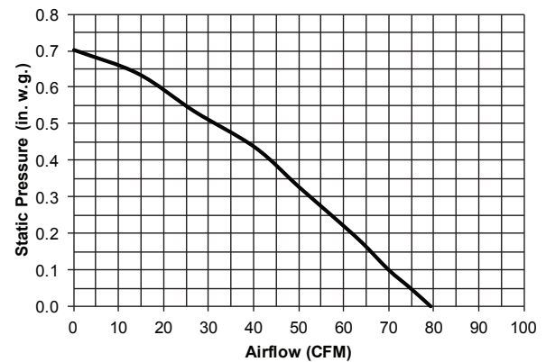
MODEL EZ80N - 3" DUCT
