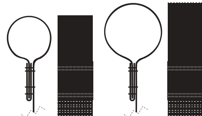
Pocket Hem Edge Extra wide, double stitched reinforced tape edge is folded over and double stitched again to create a pocket hem Options: 3" Pocket (max pipe OD = 1.029") 4" Pocket (max pipe OD = 1.660")
