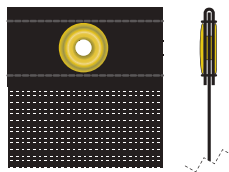
Grommet Edge Double stitched extra wide reinforced tape edge and #2 grommets (5/16" hole) Choose 2' or 4' grommet spacing
